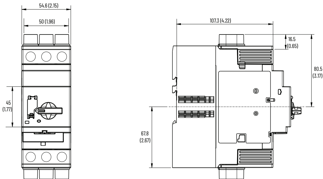
Figure 24 - Cat. No. 140MT-F-TE Type E adapter on Cat. No. 140MT-F...
