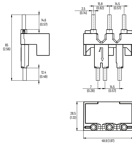
Figure 29 - Connecting Module, Cat. No. 140MT-F-PNE65
