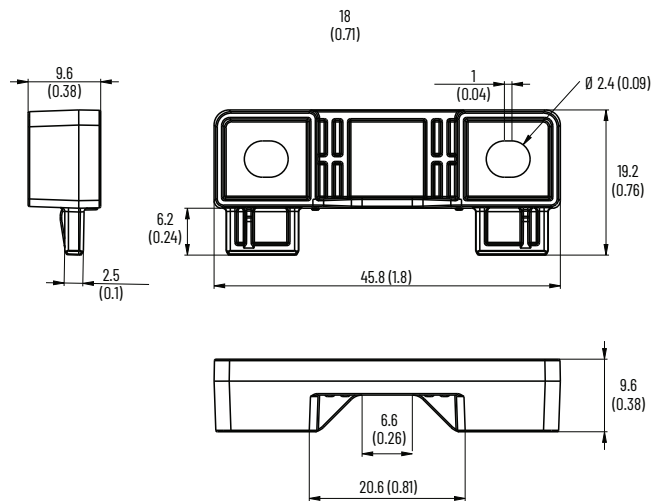
Figure 25 - Screw Adapter, Cat. No. 140MT-F-N45
