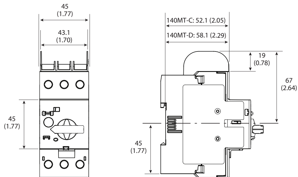
Figure 19 - 140MT-C and 140MT-D with Cat. No. 140MT-C-TE Type E Adapter
