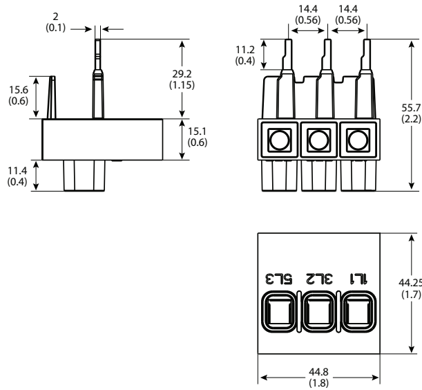
Figure 17 - Feeder Terminal for Compact Busbar, Cat. No. 140MT-C-WTEN
