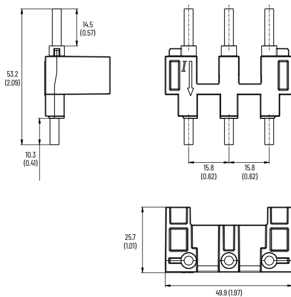
Figure 27 - Connecting Module, Cat. No. 140MT-F-PNC55
