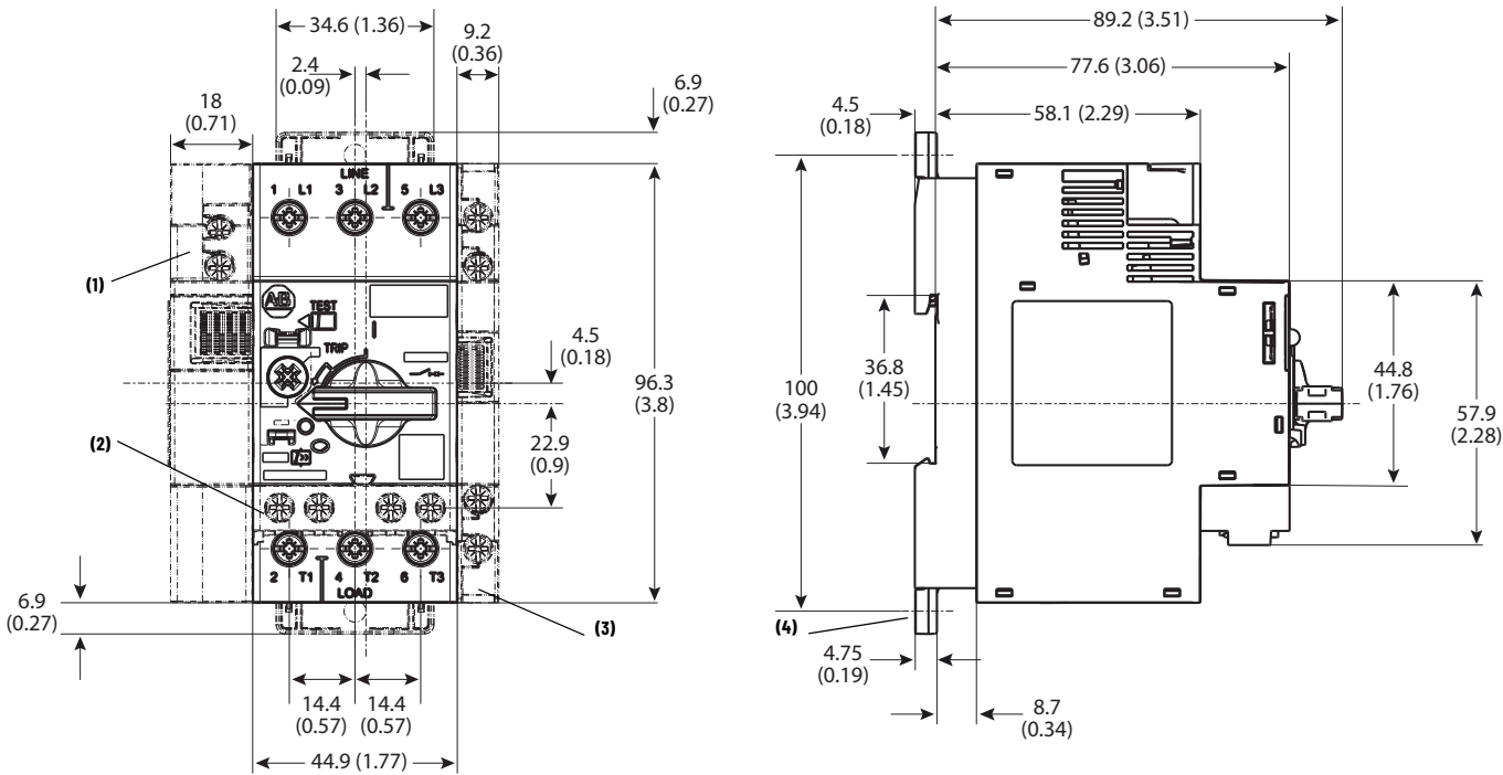
Figure 16 - Motor Protection Circuit Breaker (D-Frame), Cat. No. 140MT-D9...
