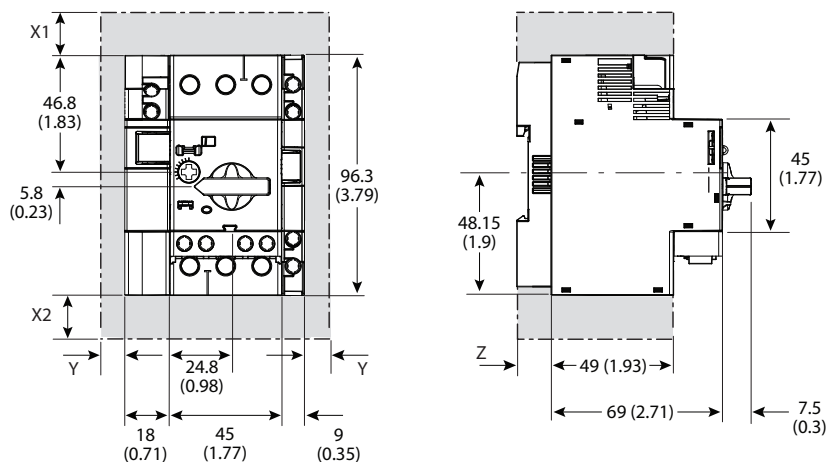
Figure 14 - Spacing Requirements
