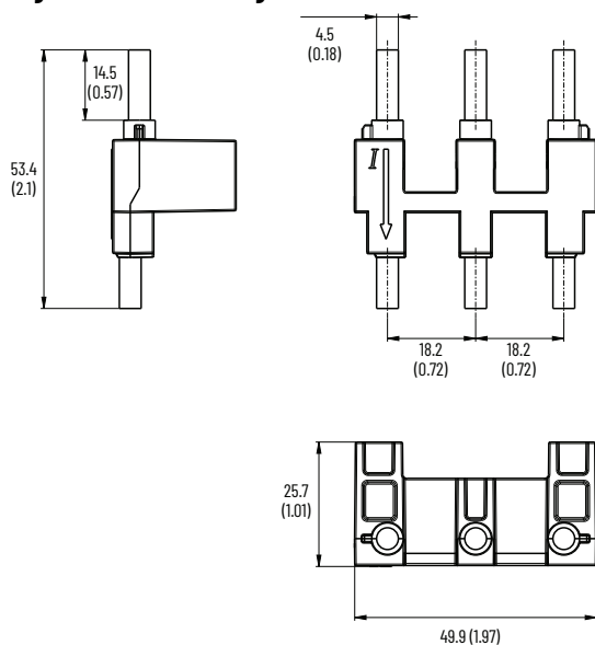
Figure 27 - Connecting Module, Cat. No. 140MT-F-PNC55
