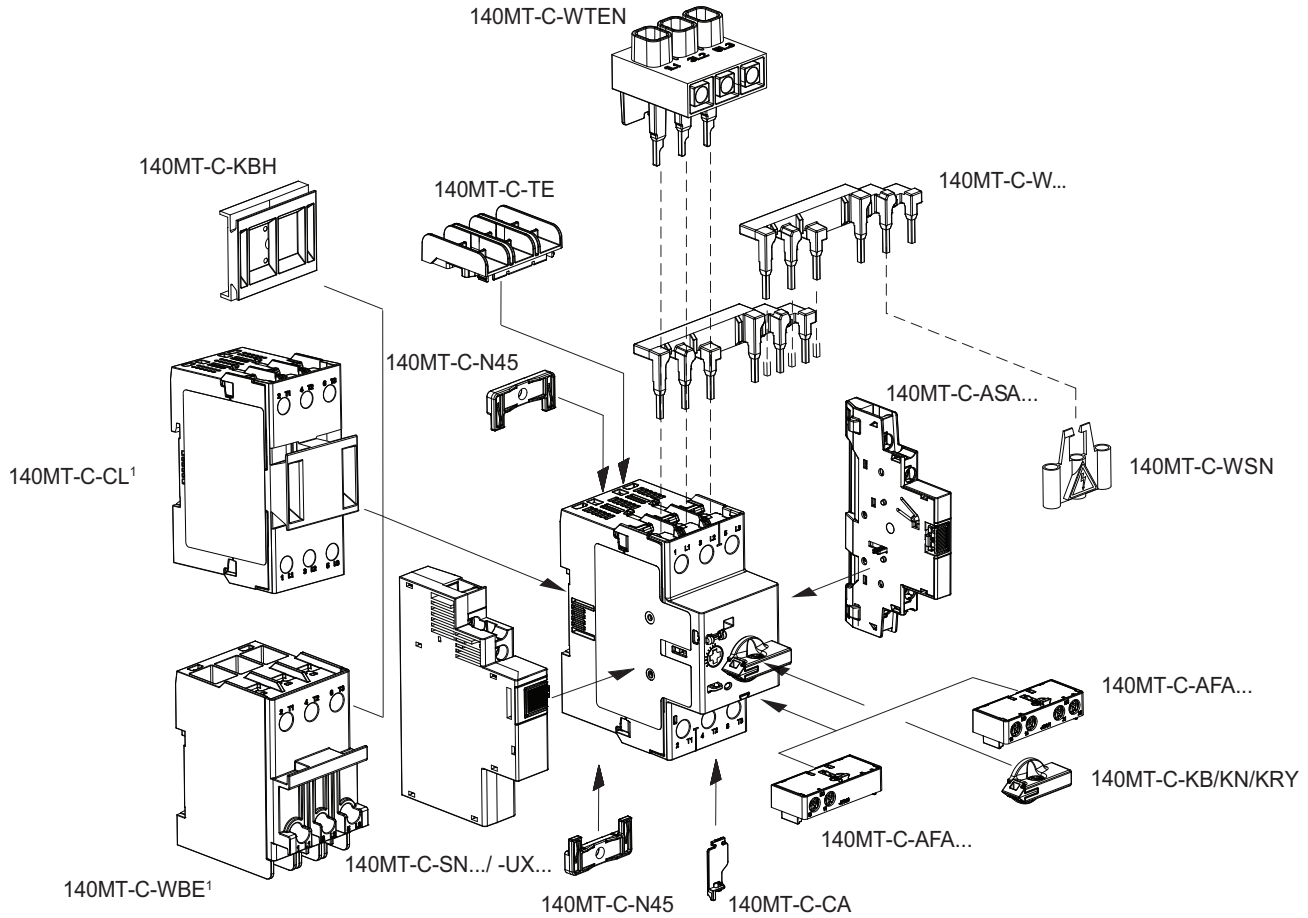
Figure 12 - Assembly Diagram
