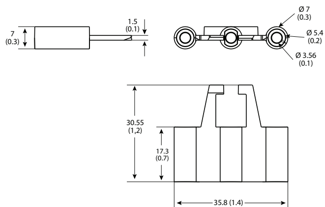
Figure 19 - 140MT-C and 140MT-D with Cat. No. 140MT-C-TE Type E Adapter
