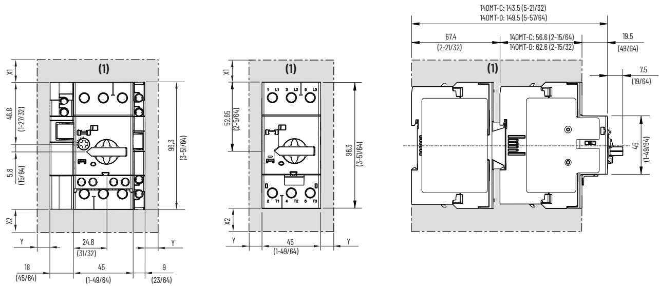
Figure 20 - Current Limiter, Cat. No. 140MT-D-CL
