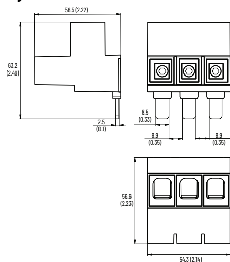
Figure 30 - Feeder Terminal, Cat. No. 140MT-F-WTE
