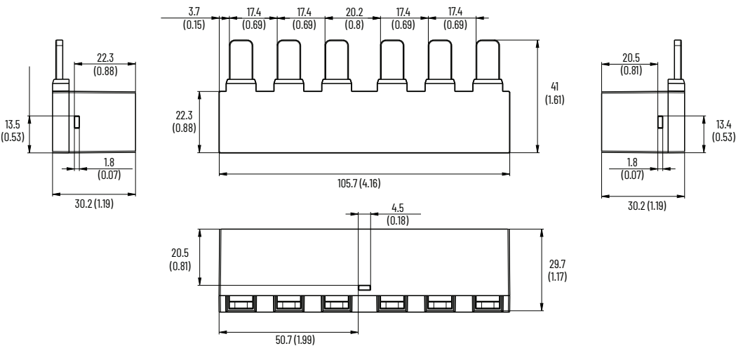
Figure 34 - Compact Busbar, Cat. No. 140MT-F-W553
