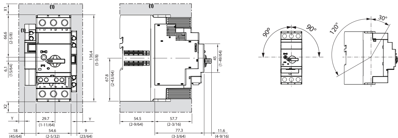
Figure 22 - Mounting Position/Safety Clearance
