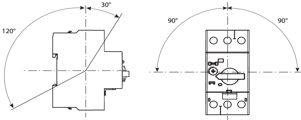
Figure 13 - Mounting Position
