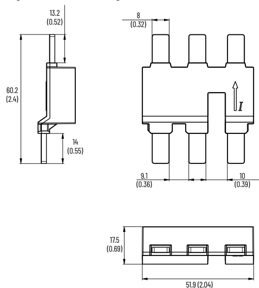
Figure 30 - Feeder Terminal, Cat. No. 140MT-F-WTE
