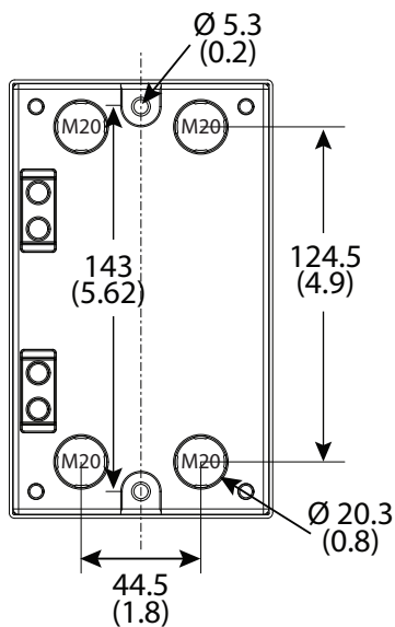
Figure 36 - Drilling Template for 140MT-C-ENRY, 140MT-C-ENN Plastic Enclosures
