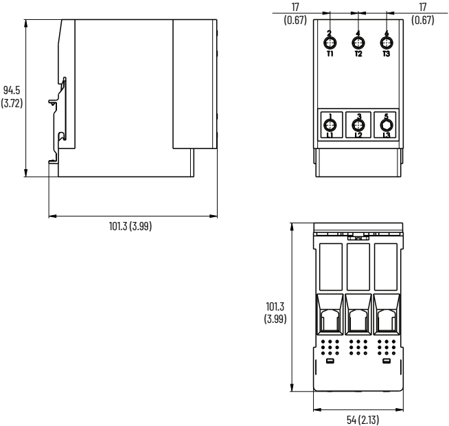
Figure 33 - Compact Busbar, Cat. No. 140MT-F-W552
