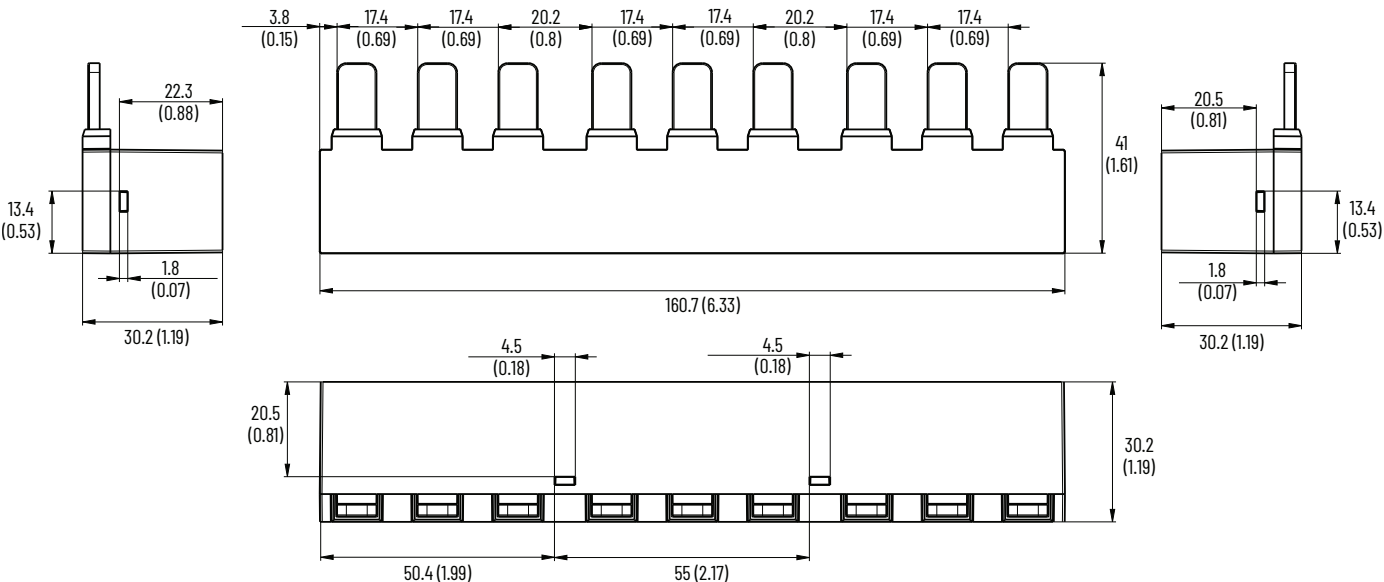
Figure 34 - Compact Busbar, Cat. No. 140MT-F-W553
