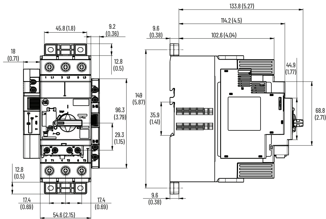
Figure 23 - Motor Protection Circuit Breaker, Cat. No. 140MT-F...
