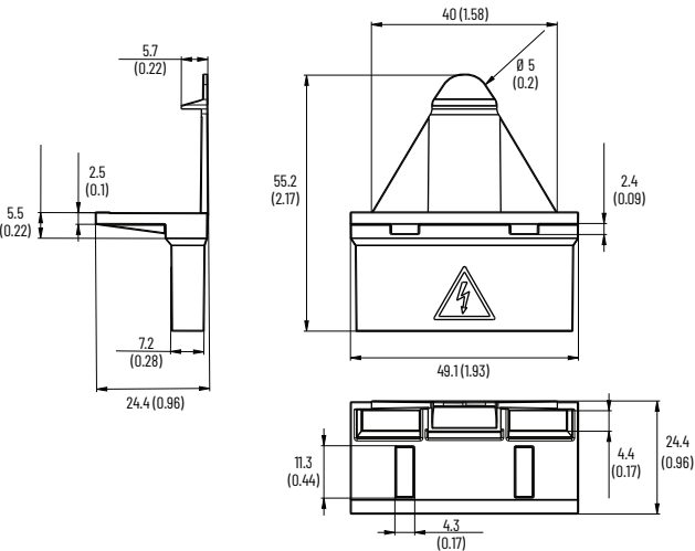
Figure 32 - Compact Bus Bar Terminal Cover, Cat. No. 140MT-F-WSN
