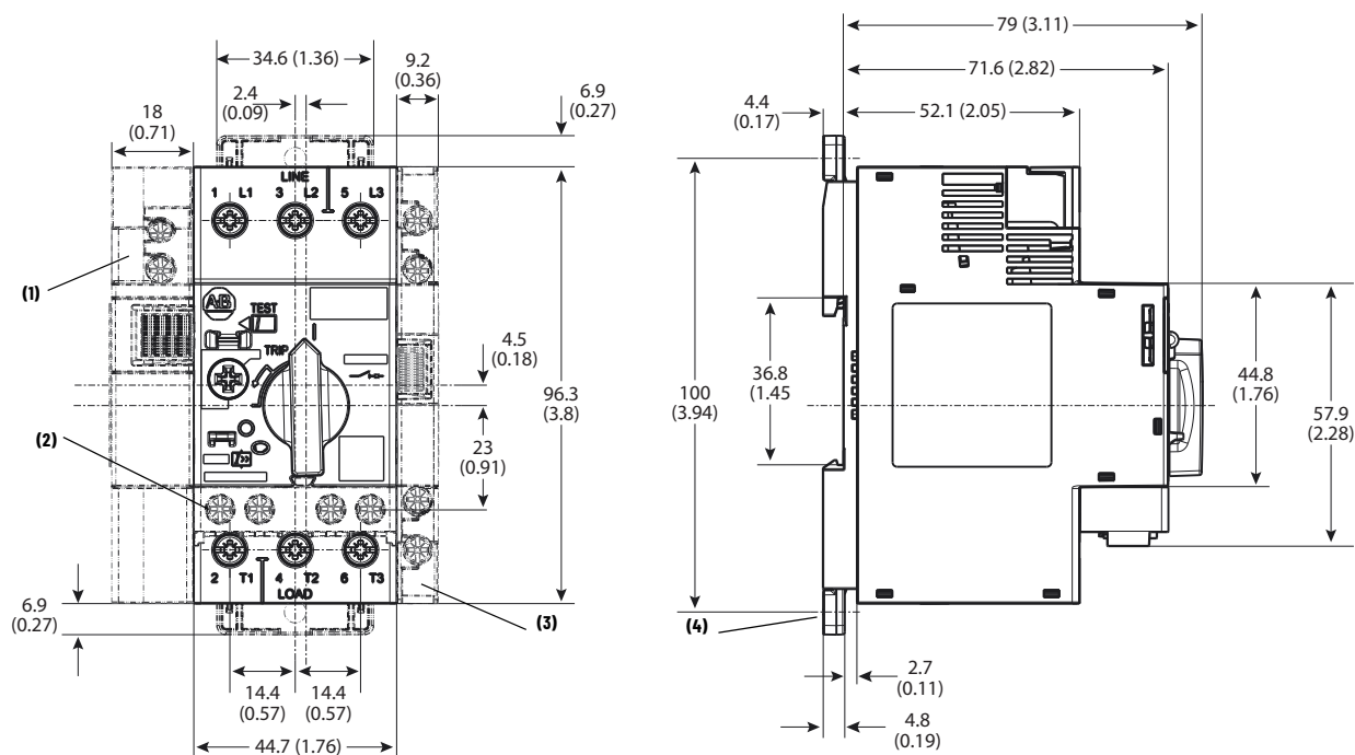
Figure 15 - Motor Protection Circuit Breaker (C-Frame), Cat. No. 140MT-C3...
