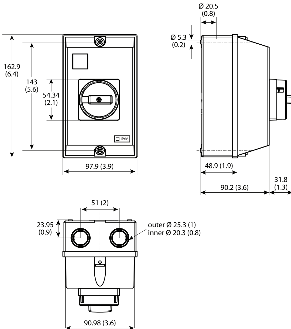
Figure 35 - 140MT-C-ENRY, 140MT-C-ENN Plastic Enclosures
